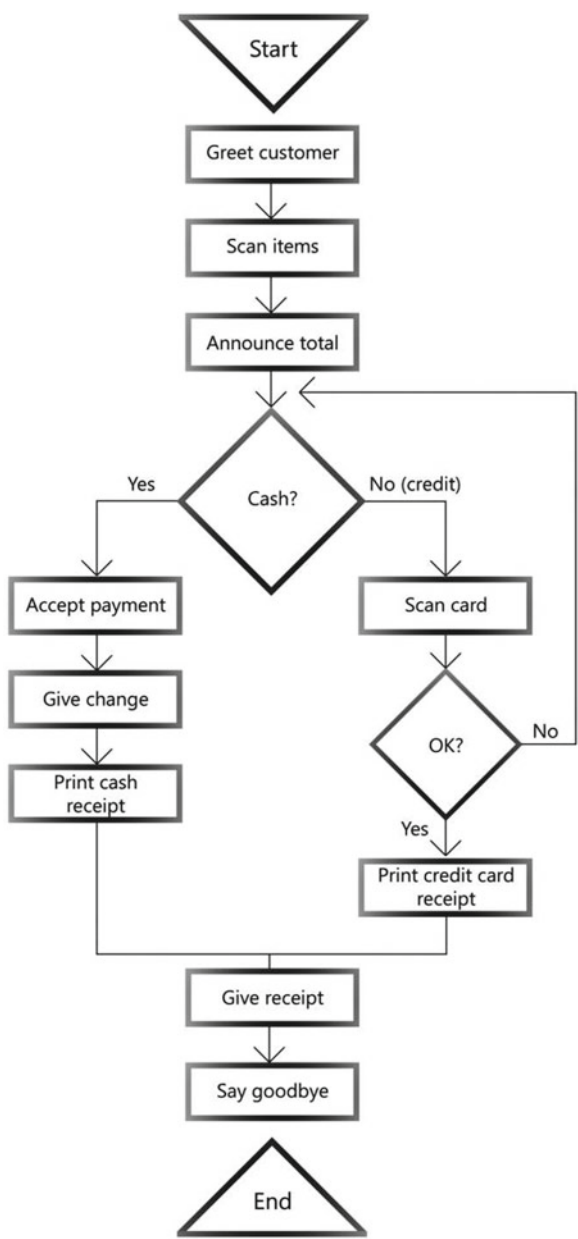
Figure 5-1. Flowchart for store checkout
